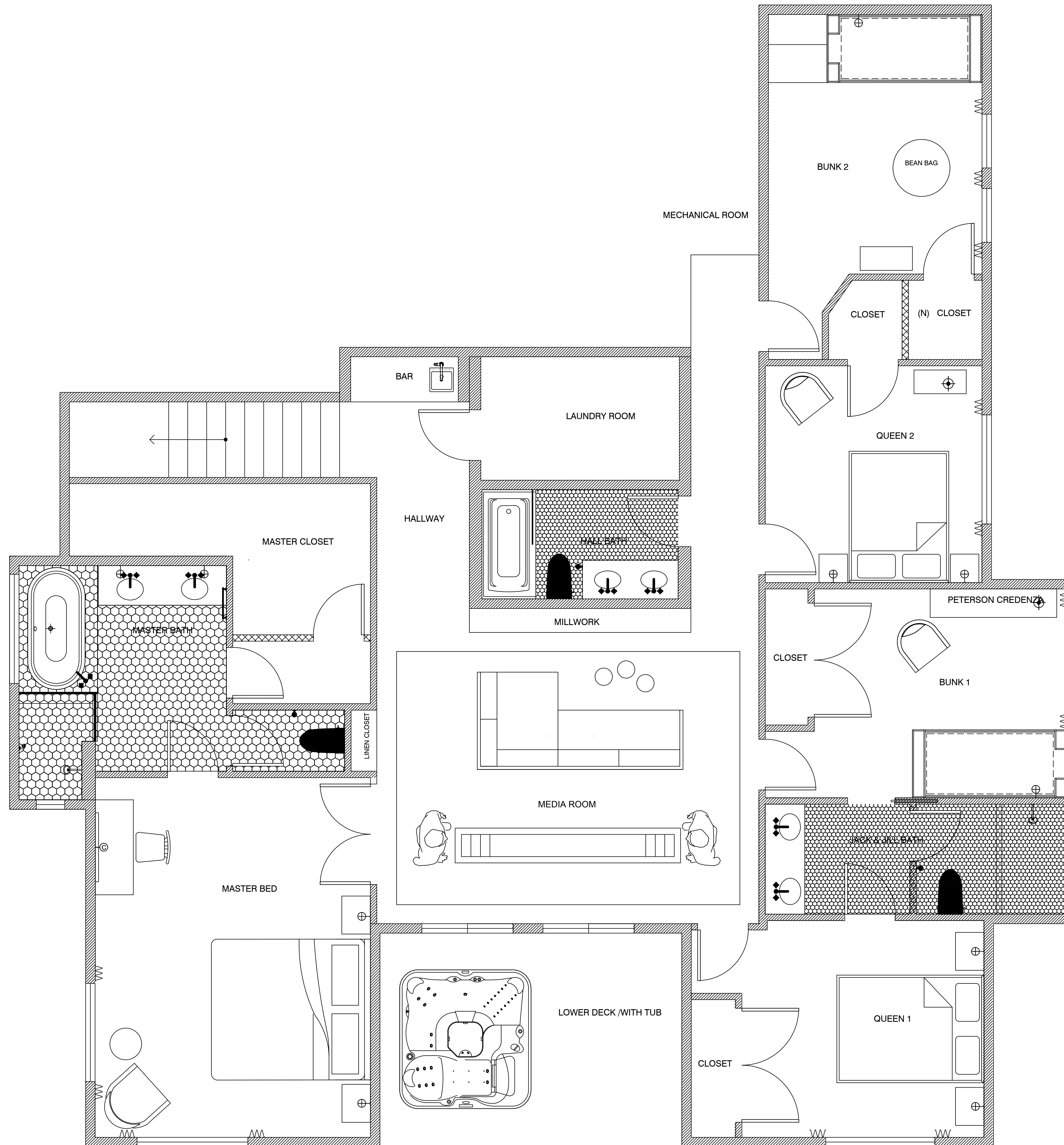
1 LOWER LEVEL - PLAN
